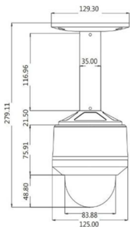
■ Hoisting installation dimensions
