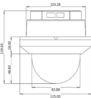
■ Wall installation dimensions
