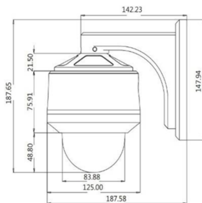
■ Wall installation dimensions
