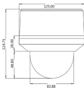
■ Hoisting installation dimensions
