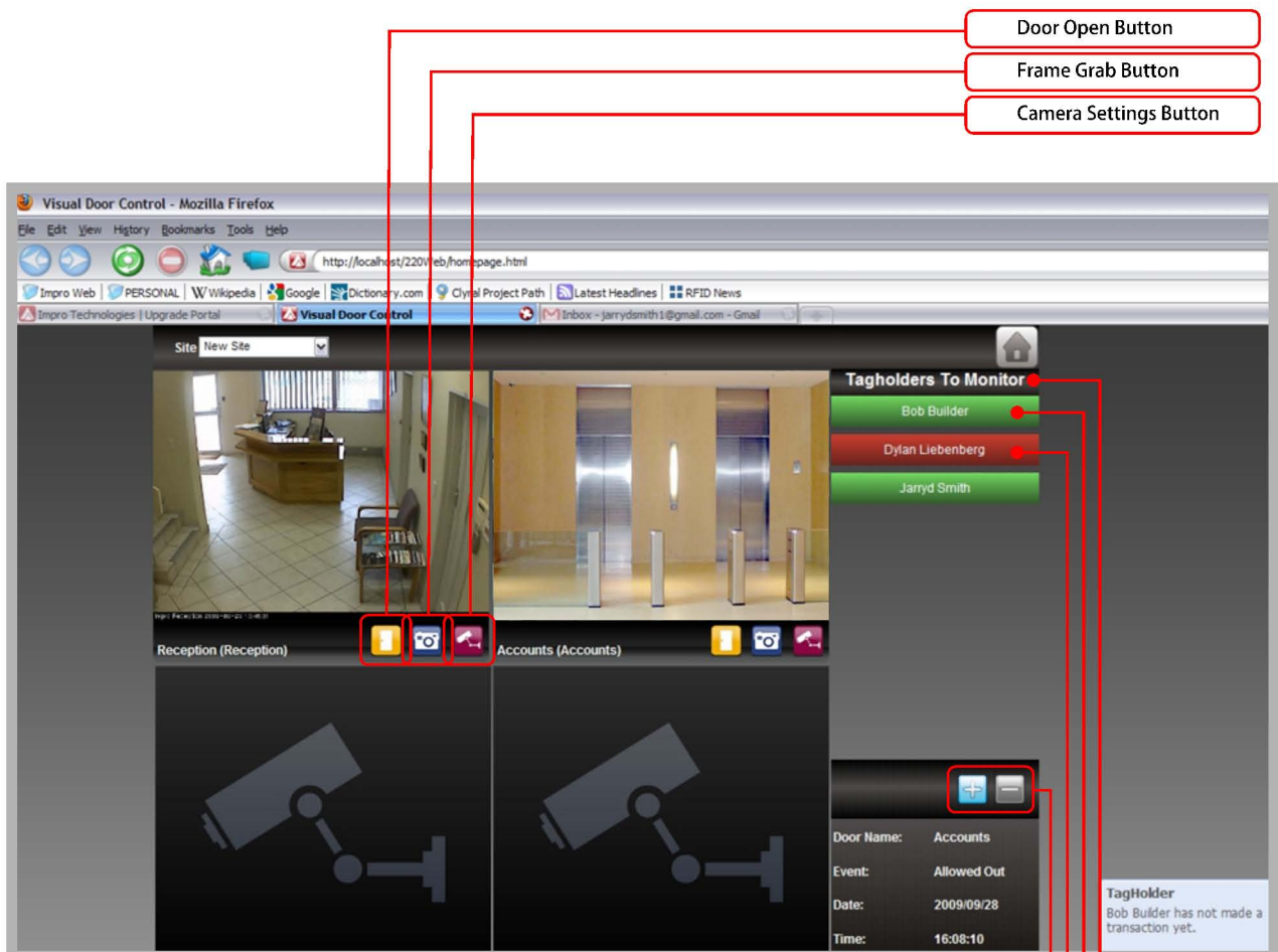
[image: Visual Door Control with two active cameras, monitoring three Tagholders]
