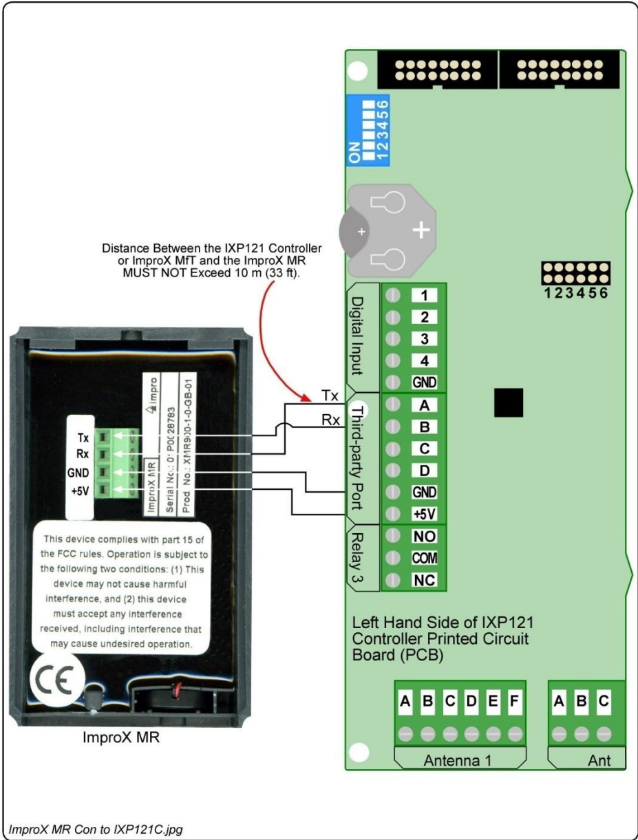
Figure 1: ImproX MR Connected to the IXP121 Controller or ImproX Mft
