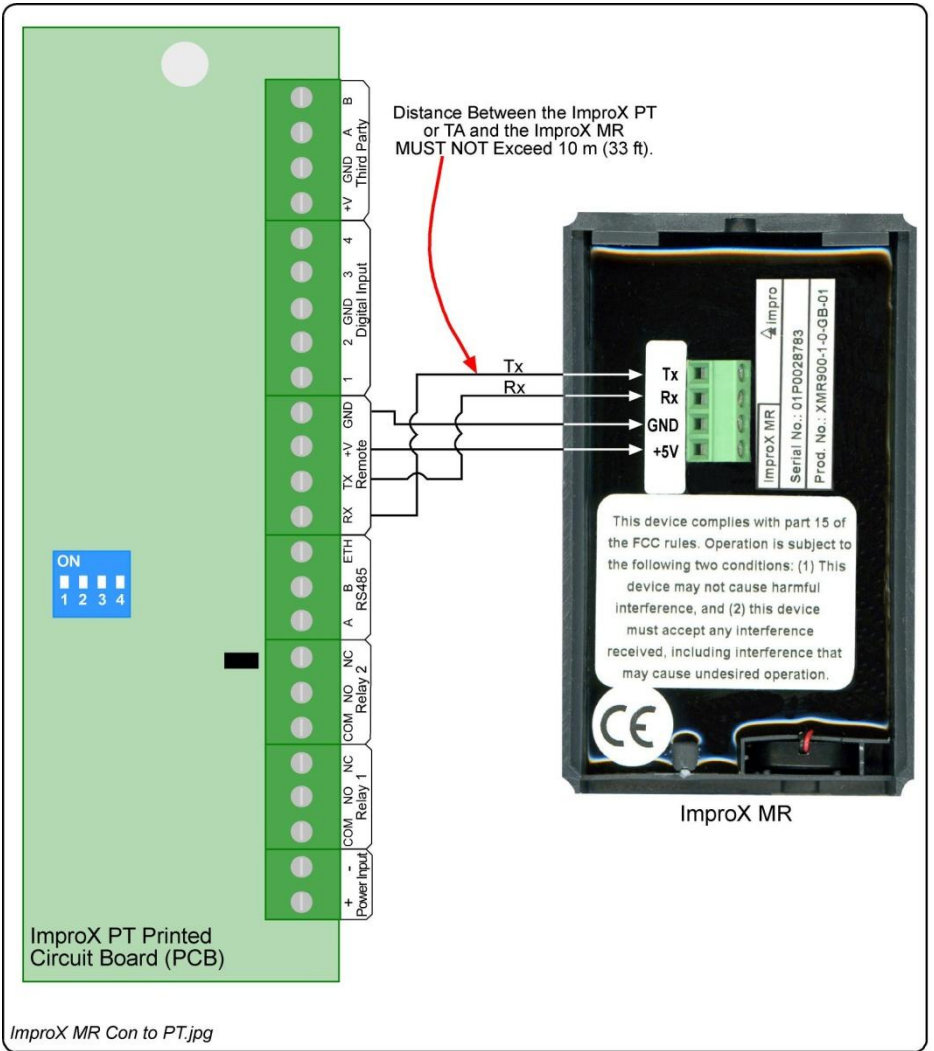
Figure 2: ImproX MR Connected to the ImproX PT or ImproX TA
