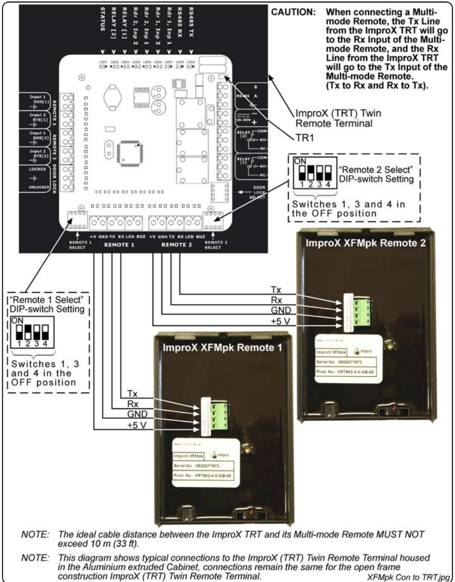
Figure 1: ImproX XFMpk Connected to the ImproX TRT
