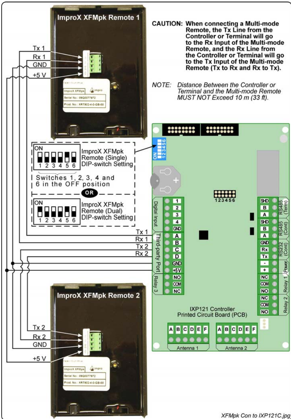
Figure 2: ImproX XFMpk Connected to the IXP121 Controller or ImproX MfT
