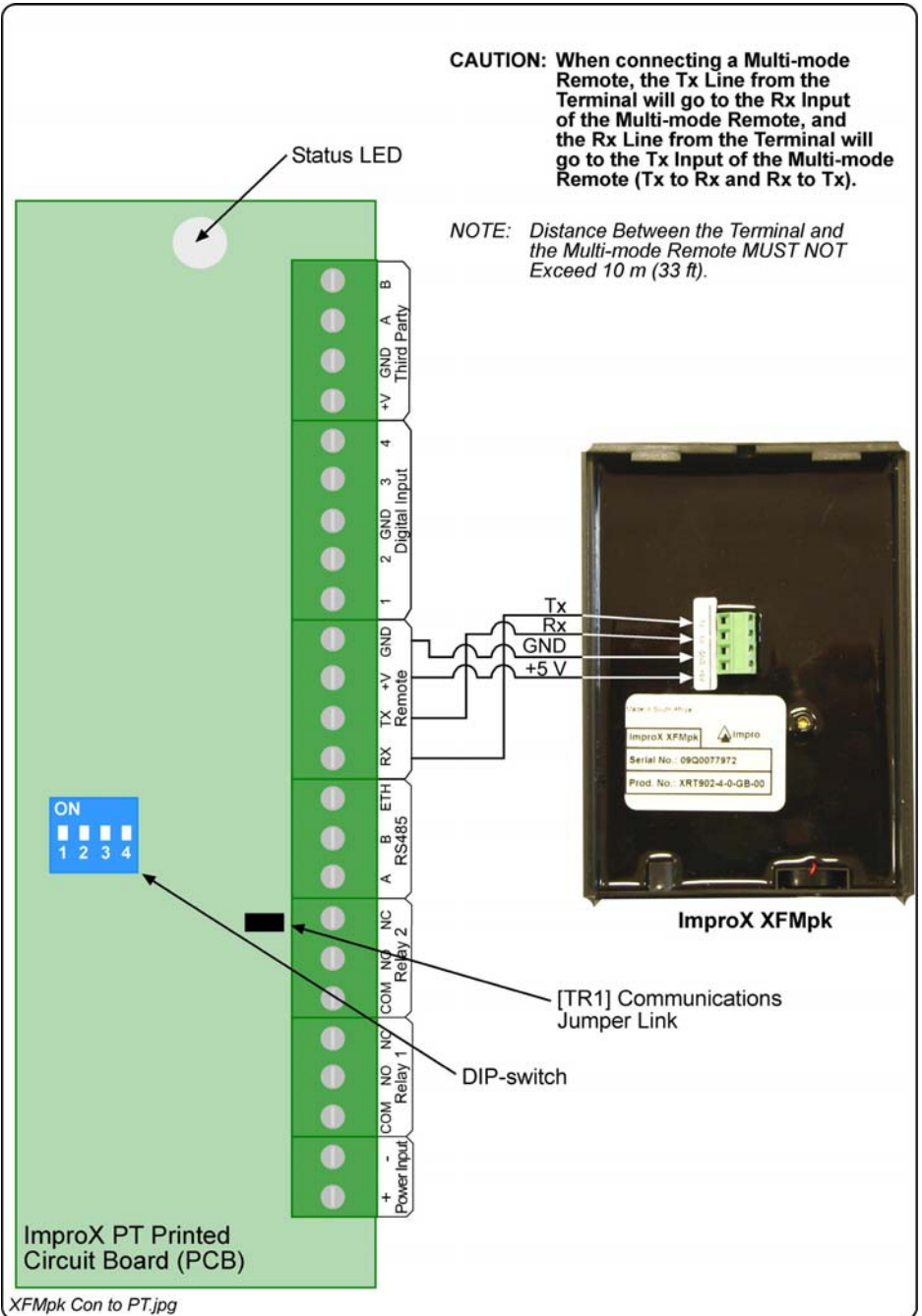
Figure 3: ImproX XFMpk Connected to the ImproX PT or ImproX TA
