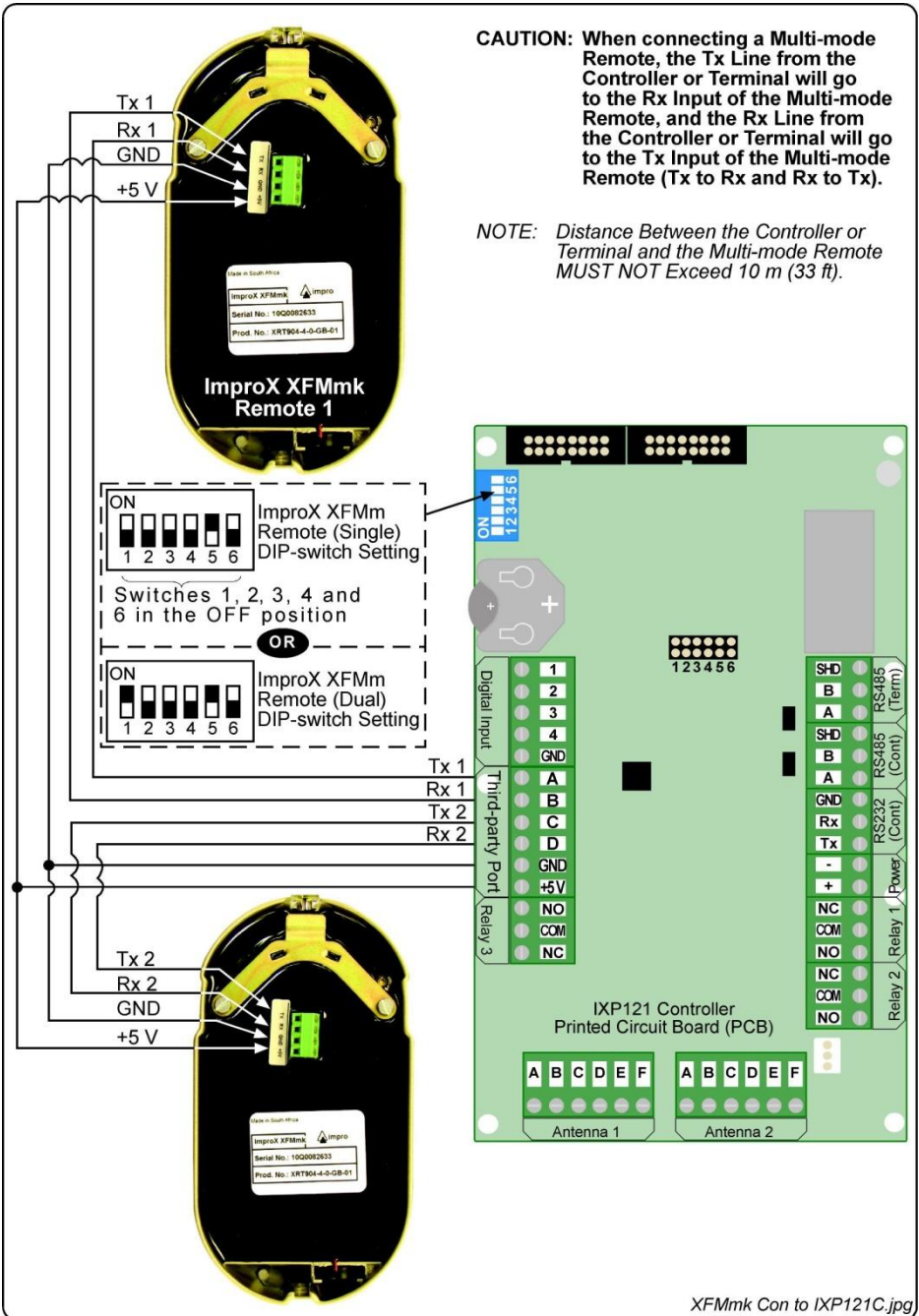
Figure 2: ImproX XFMmk Connected to the IXP121 Controller or ImproX Mft
