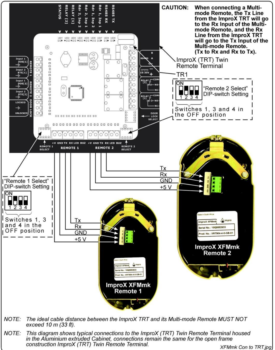
Figure 1: ImproX XFMmk Connected to the ImproX TRT
