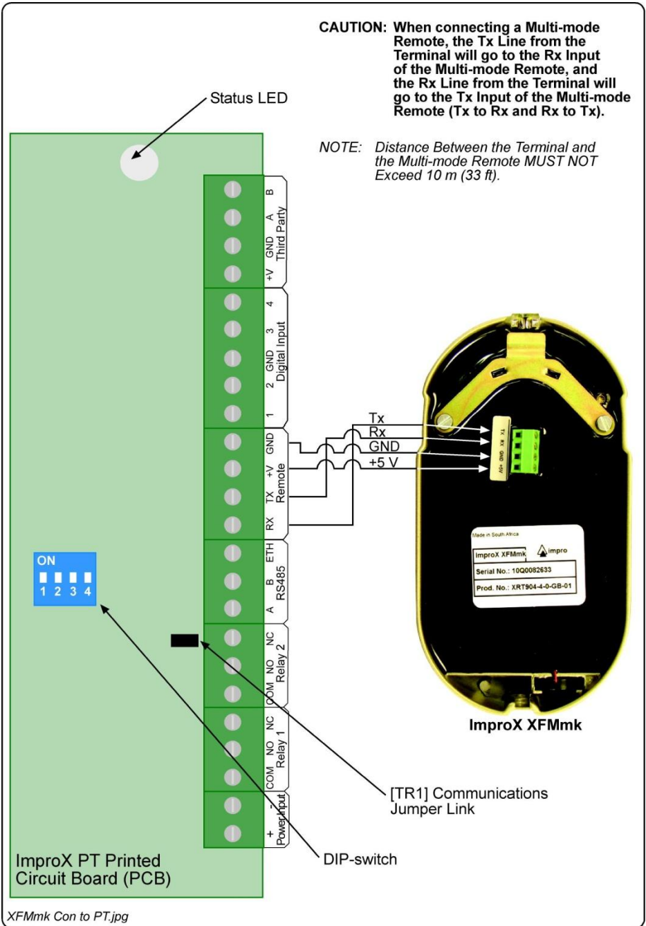
Figure 3: ImproX XFMmk Connected to the ImproX PT or ImproX TA
