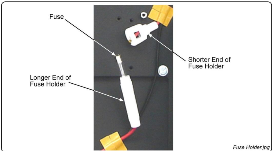
Figure 5: Fuse Holder
