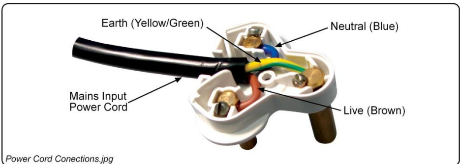
Figure 4: Mains Plug Connections
