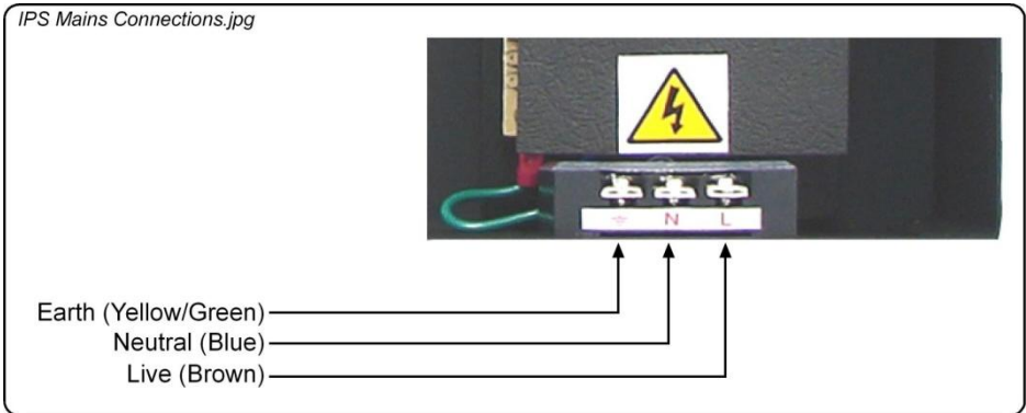
Figure 3: IPS Mains Connections
