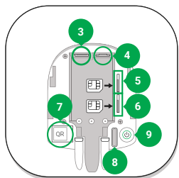
3 - Power supply cable socket 4 - Ethernet cable socket 5 - Slot 2: backup SIM card (micro-SIM type) 6 - Slot 1: main SIM card (micro-SIM type) 7 - QR code 8 - Tamper button 9 - Power button
