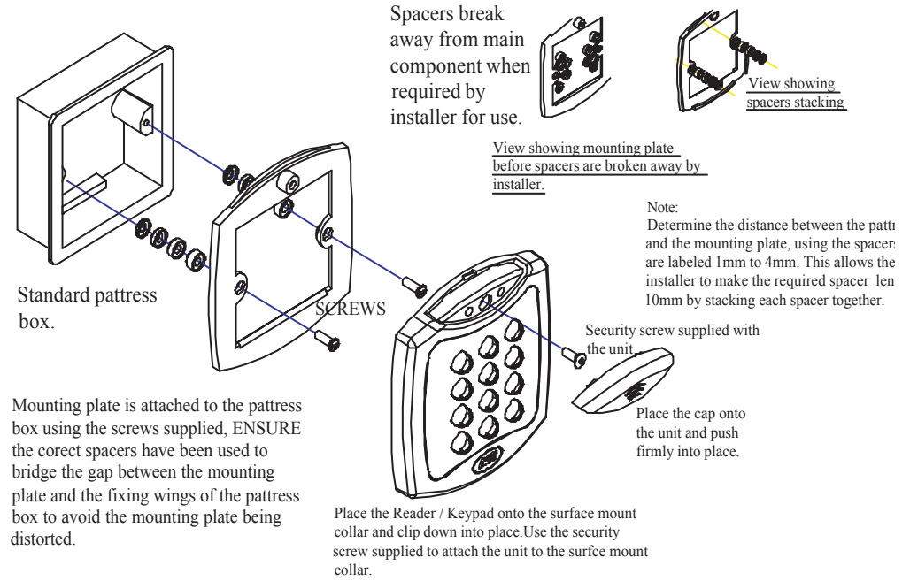
Fig 2 Mounting instructions for flush mount unit
