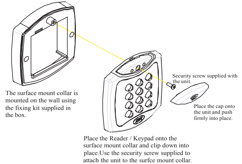
Fig 3 Mounting instructions for surface mount unit
